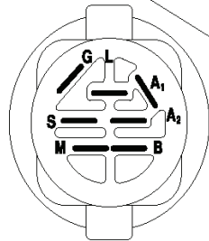
IGNITION SWITCH
